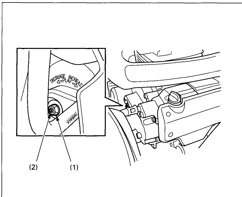
Fig. 4-16 (1) Lock nut
